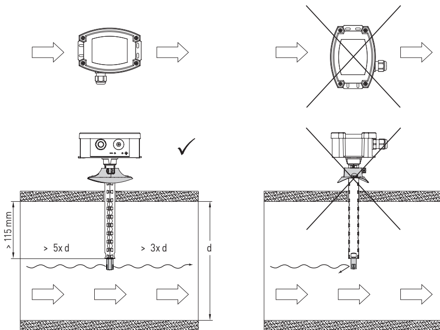
Mounting diagram
