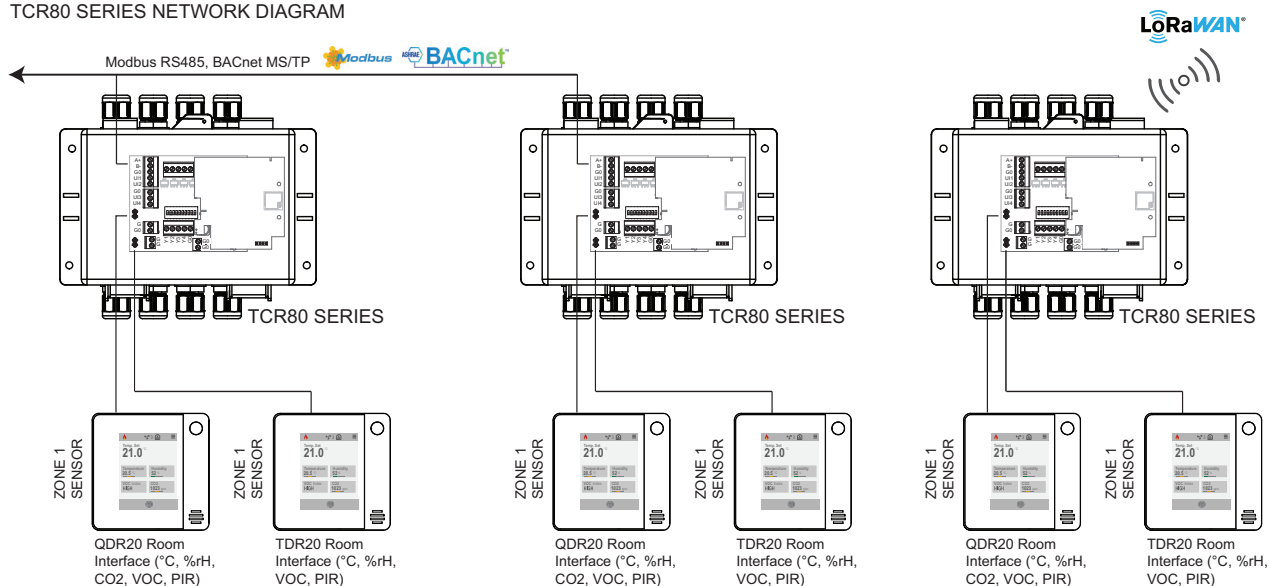
TCR80 SERIES NETWORK DIAGRAM
